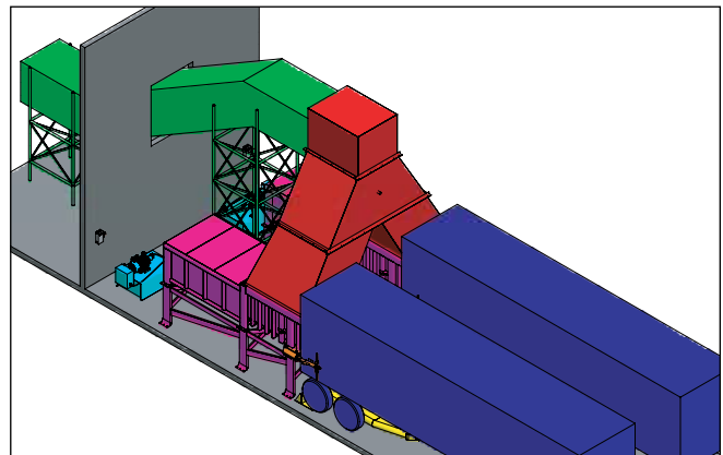
Tandem CP-8002 units being loaded by a conveyor system, and packing into transfer trailers
